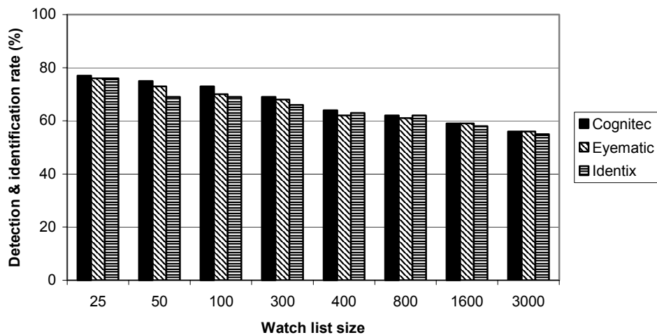
Figure 8. Watch list performance is shown for the three best systems on the HCInt visa dataset. Detection and identification rates are reported at a false alarm rate of 1% for eight watch list sizes.
